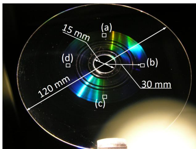
Figure 2. Photograph of injection-compression-molded replica (this photograph shows a replica mold fabricated under the condition COP-1). Indicated areas 30 mm from the center (a–d) show the regions at which the uniformity of the degree of replication by UV-NIL is examined.
