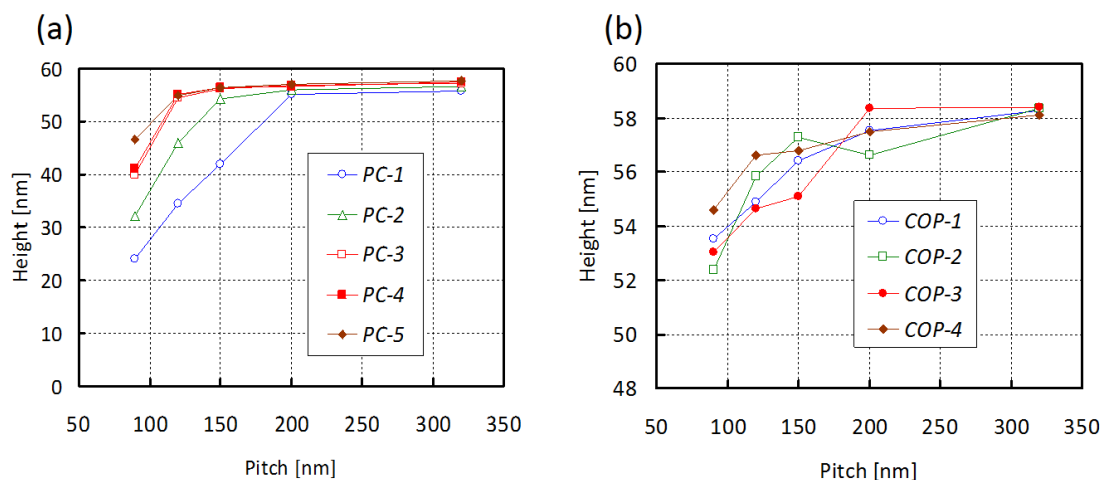
Figure 3. Pattern heights of injection-compression-molded replicas of samples (a) PC-1-5 and (b) COP-1-4 obtained by atomic force microscopy (AFM) analyses as a function of pattern pitches.
