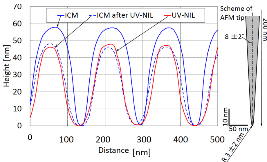
Figure 5. AFM images of the 150-nm-pitch patterns of injection-compression-molded replica (sample COP-1), after use in UV-NIL, and UV-cured resist. The scheme of AFM tip used is illustrated with the same scale of the graph.
